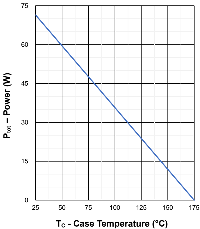
Fig 1. Power Capability
