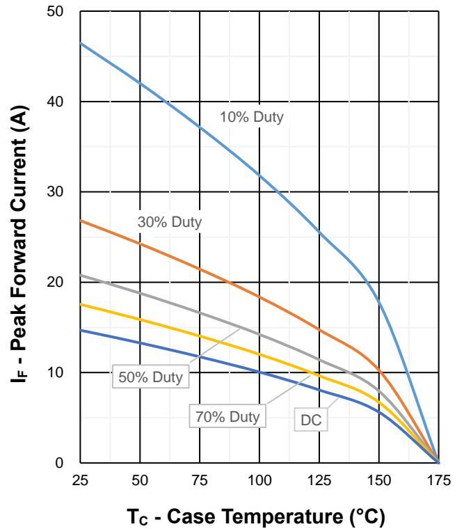
Fig 2. Current Capability
