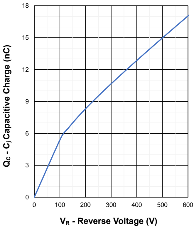
Fig 7. Capacitance Charge
