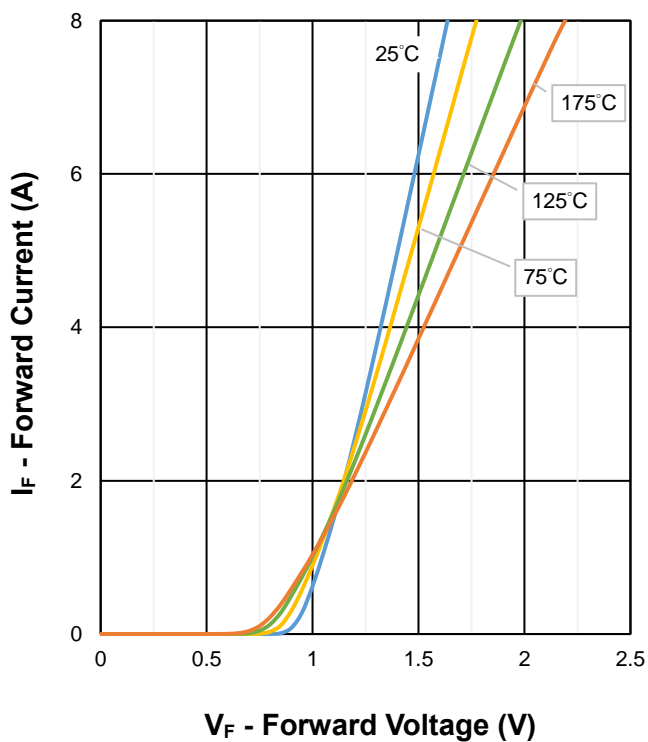
Fig 3. Forward Characteristics
