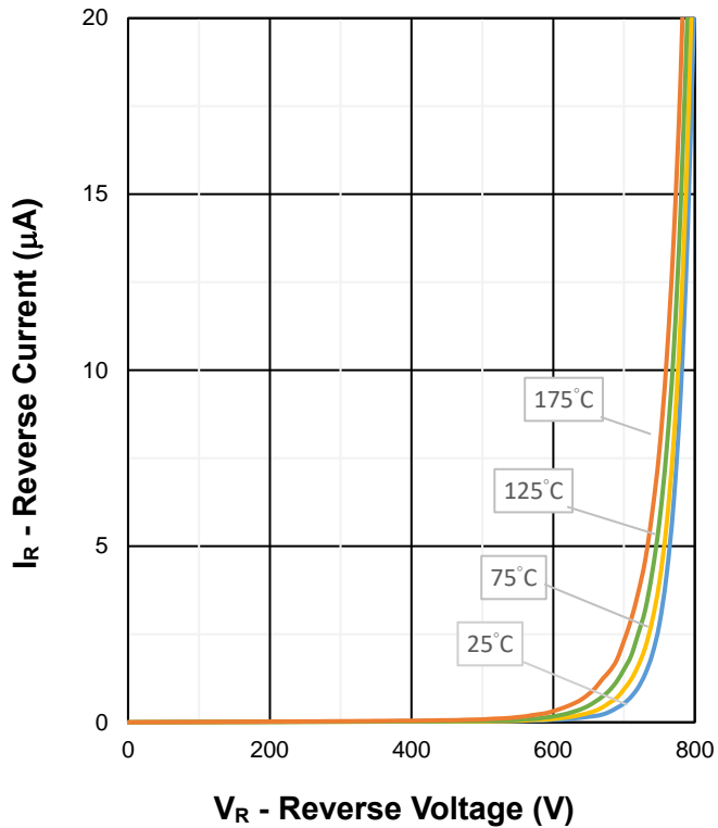
Fig 5. Reverse Characteristics
