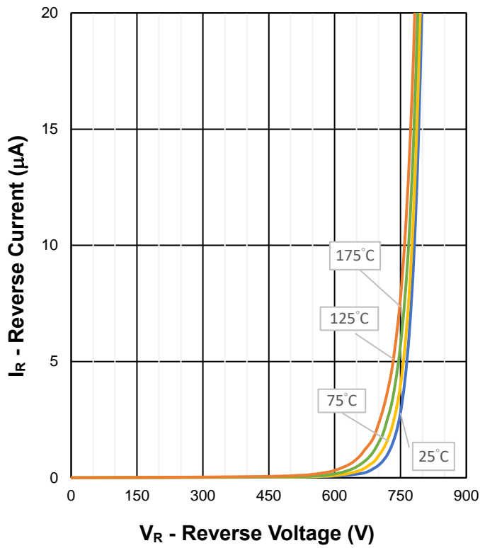
Fig 5. Reverse Characteristics
