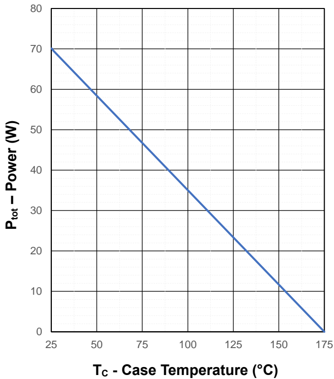
Fig 1. Power Capability
