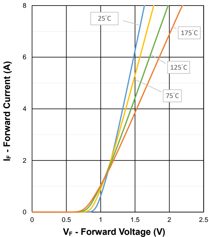
Fig 3. Forward Characteristics
