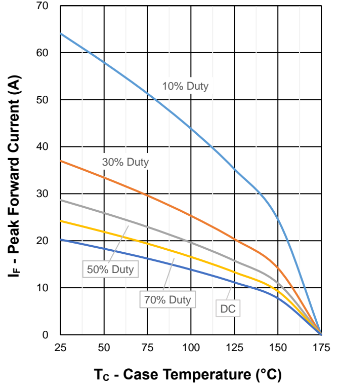
Fig 2. Current Capability
