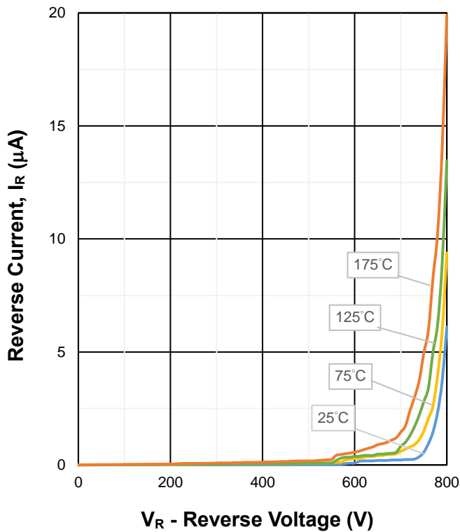
Fig 5. Reverse Characteristics
