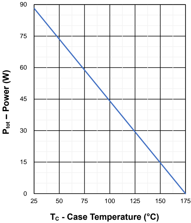
Fig 1. Power Capability
