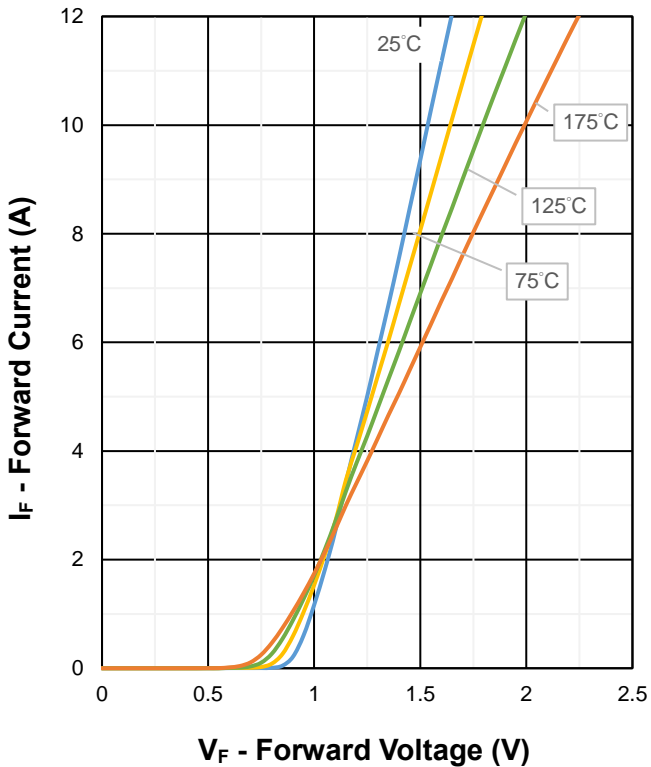
Fig 3. Forward Characteristics
